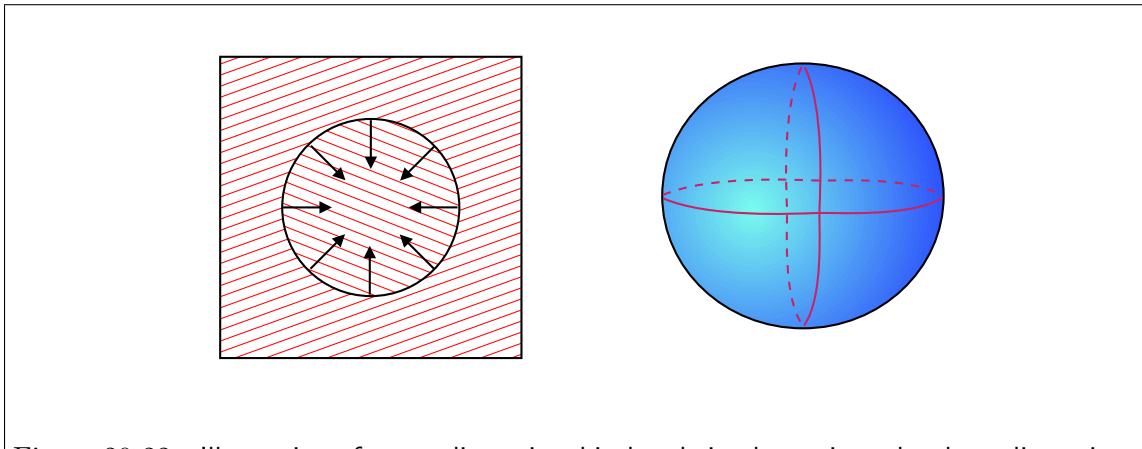
Figure 20-22: Illustration of a two-dimensional isolated circular grain and a three-dimensional isolated spherical grain. Because there is an extra energy in the system \Delta G_{2D} = 2\pi R\gamma_{gb} and \Delta G_{3D} = 4\pi R^2\gamma_{gb} , there is a driving force to reduce the radius of the grain. A simple model for grain growth is that the velocity (normal to itself) of the grain boundary is v_{gb} = M_{gb}\gamma_{gb}\kappa where M_{gb} is the grain boundary mobility and \kappa is the mean curvature of the boundary. The normal velocity v_{gb} is towards the center of curvature.
