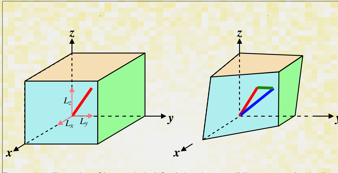
Figure 10-7: Illustration of how strain is defined: imagine a small line-segment that is aligned with a particular direction (one set of indices for the direction of the line-segment); after deformation the end-points of the line segment define a new line-segment in the deformed state. The difference in these two vectors is a vector representing how the line segment has changed from the initial state into the deformed state. The difference vector can be oriented in any direction (the second set of indices)—the strain is a representation of “a difference vectors for all the oriented line-segments” divided by the length of the original line.
