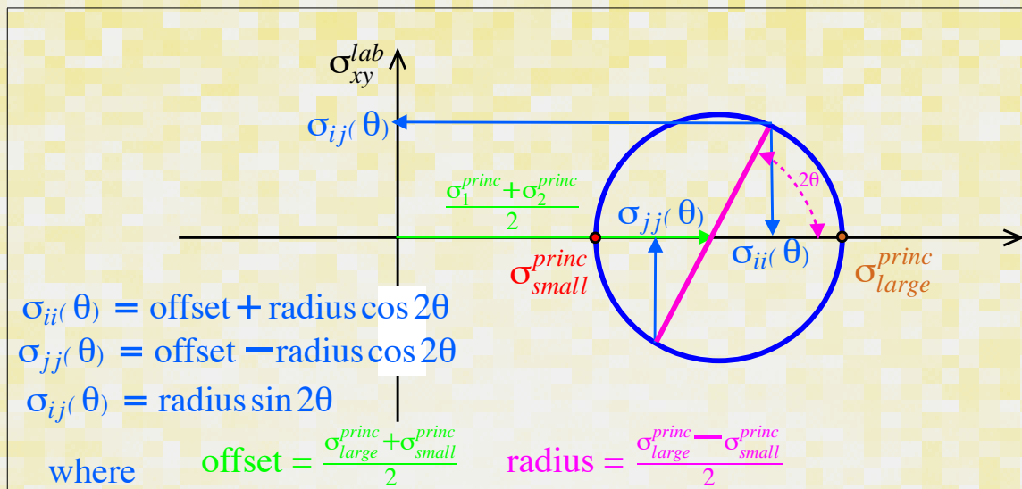
Figure 10-8: Mohr's circle of stress is a way of graphically representing the two-dimensional stresses of identical stress states, but in rotated laboratory frames. The center of the circle is displaced from the origin by a distance equal to the average of the principal stresses (or average of the eigenvalues of the stress tensor). The maximum and minimum stresses are the eigenvalues—and they define the diameter in the principal \theta = 0 frame. Any other point on the circle gives the stress tensor in a frame rotated by 2\theta from the principal axis using the construction illustrated by the blue lines (and equations).
