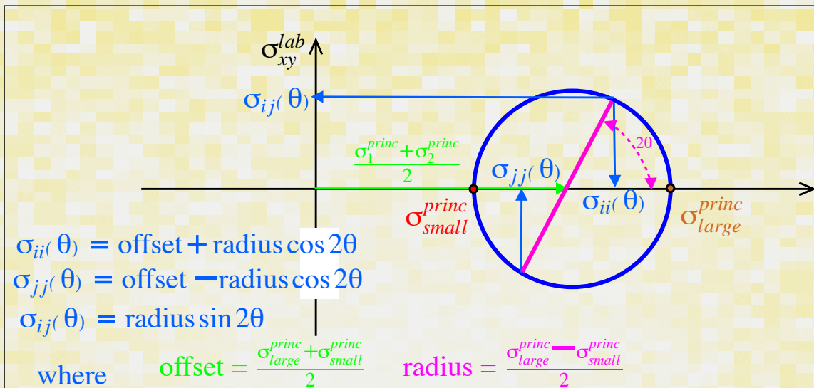
Figure 10-8: Mohr's circle of stress is a way of graphically representing the two-dimensional stresses of identical stress states, but in rotated laboratory frames.
