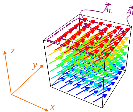
Figure 16-16: Illustration of a vector “flow field” \vec{J} near a point in three dimensional space. If each vector represents the rate of “stuff” flowing per unit area of a plane that is normal to the direction of flow, then the dot product of the flow field integrated over a planar oriented area \vec{A} is the rate of “stuff” flowing through that plane. For example, consider the two areas indicated with purple (or dashed) lines. The rate of “stuff” flowing through those regions is \vec{J} \cdot \vec{A}_B = \vec{J} \cdot \hat{k} A_B and \vec{J} \cdot \vec{A}_L = \vec{J} \cdot \hat{k} A_L .
