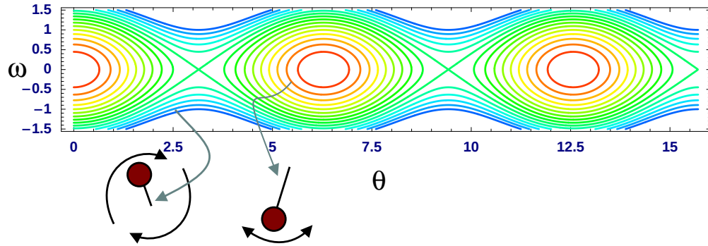
Figure 25-1: Example of the phase plane for the pendulum equation. The small closed orbits are the stable harmonic oscillations about the stable position \bullet . The larger orbits are those with increasing energy until the energy is just large enough that the pendulum rises to its unstable equilibrium position \bullet . The two kinds of fixed points (i.e., the stable and unstable points where \dot{\omega} = \dot{\theta} = 0 ) regulate the portrait of the phase plane. (Note: The word “phase” here should not be confused with the common usage of phase in materials science. In the current context for example, the phase represents the positions and momenta of all the particles in a system—this usage is important in statistical mechanics. However, the word “phase” in materials science and engineering is usually interpreted as a portion of material that lies within an identifiable interface—this usage is implied in “equilibrium phase diagrams.”)
