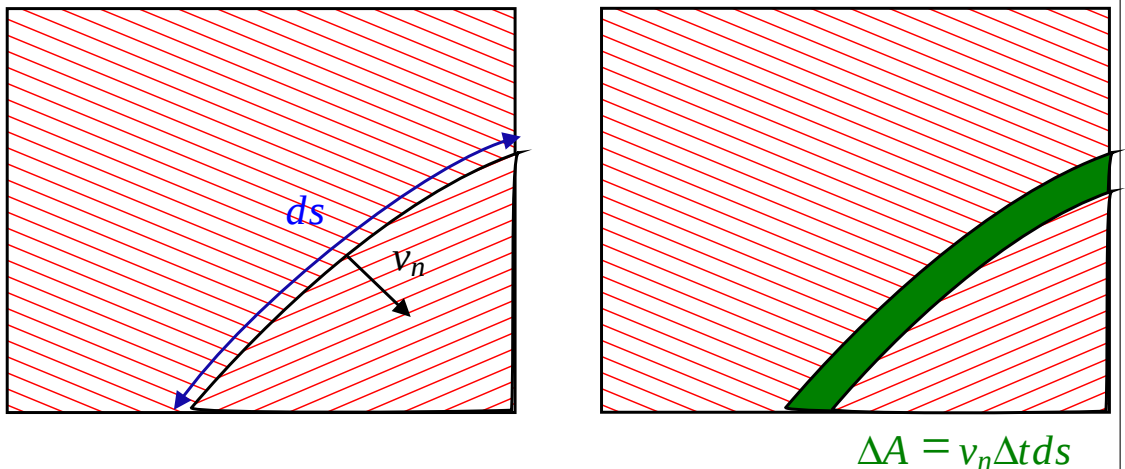
Figure 20-2: A segment of a grain boundary moving with normal velocity v_n will move a distance v_n\Delta t in a short time \Delta t . The motion will result in a change of area -\Delta A for the shrinking grain. Each segment, ds , of boundary contributes to the loss of area by \Delta A = -v_n\Delta t ds .
