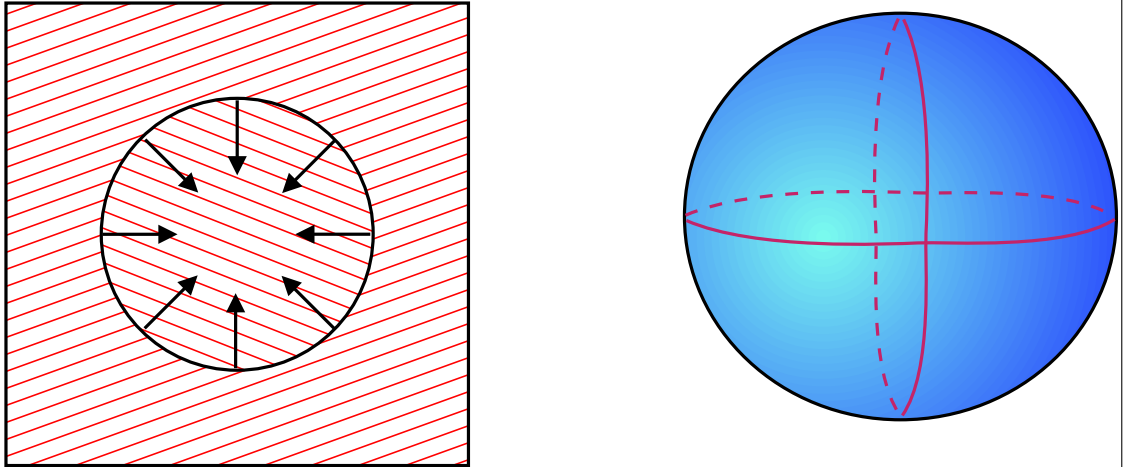
Figure 20-1: Illustration of a two-dimensional isolated circular grain and a three-dimensional isolated spherical grain. Because there is an extra energy in the system \Delta G_{2D} = 2\pi R\gamma_{gb} and \Delta G_{3D} = 4\pi R^2\gamma_{gb} , there is a driving force to reduce the radius of the grain. A simple model for grain growth is that the velocity (normal to itself) of the grain boundary is v_{gb} = M_{gb}\gamma_{gb}\kappa where M_{gb} is the grain boundary mobility and \kappa is the mean curvature of the boundary. The normal velocity v_{gb} is towards the center of curvature.
